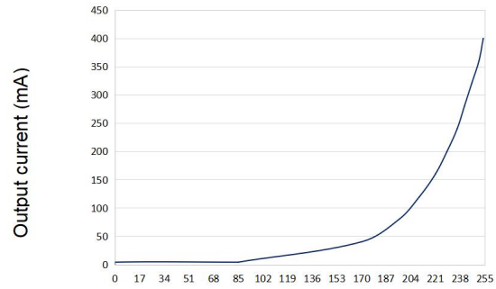
Logarithmic dimming
